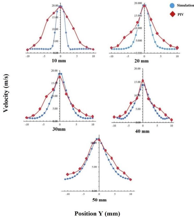
Figure 8. Velocity profiles at different points under the nozzle: numerical simulation and PIV.
