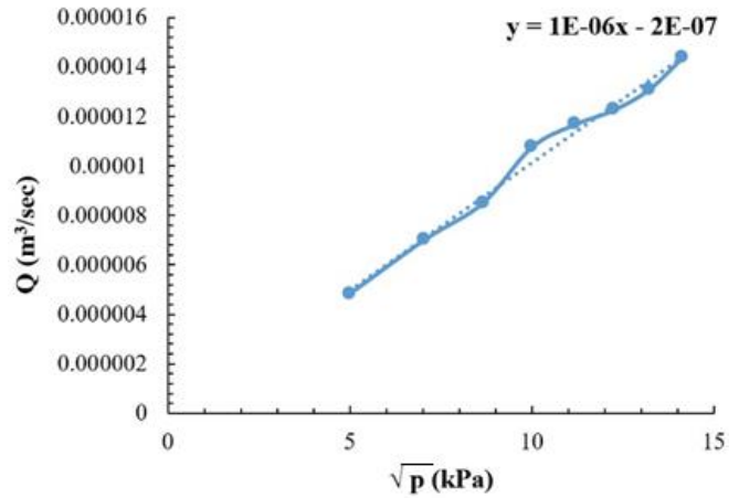
Figure 5. Coefficient of discharge for extended flat fan nozzle.
