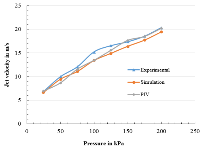
Figure 6. Comparison of jet velocity.
