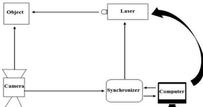
Figure 4a. Schematic diagram of Particle Image Velocimetry (PIV) system (Nadeem et al. , 2018).
