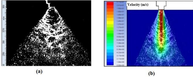
Figure 7. PIV image captured at 200 kPa (a), Overlapping of PIV and CFD images at 200 kPa.
