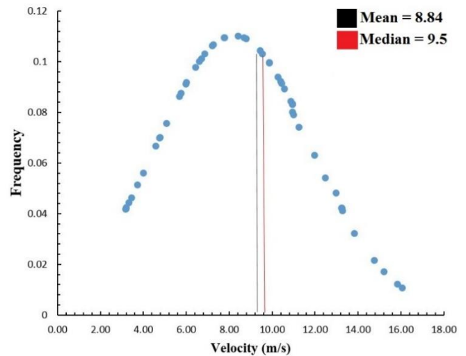
Figure 9. Velocity distribution under the sprayer nozzle at 200 kPa pressure.
