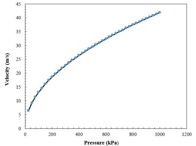
Figure 10. Jet velocity prediction at high pressure.
