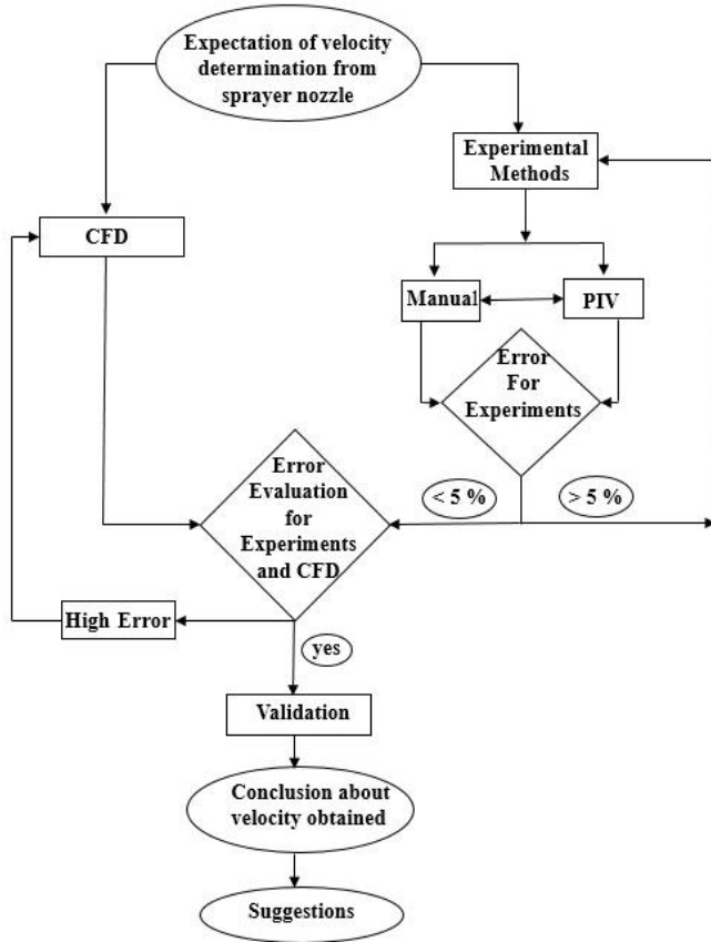
Figure 1. Schematic diagram of analysis for spray nozzle measurement.
